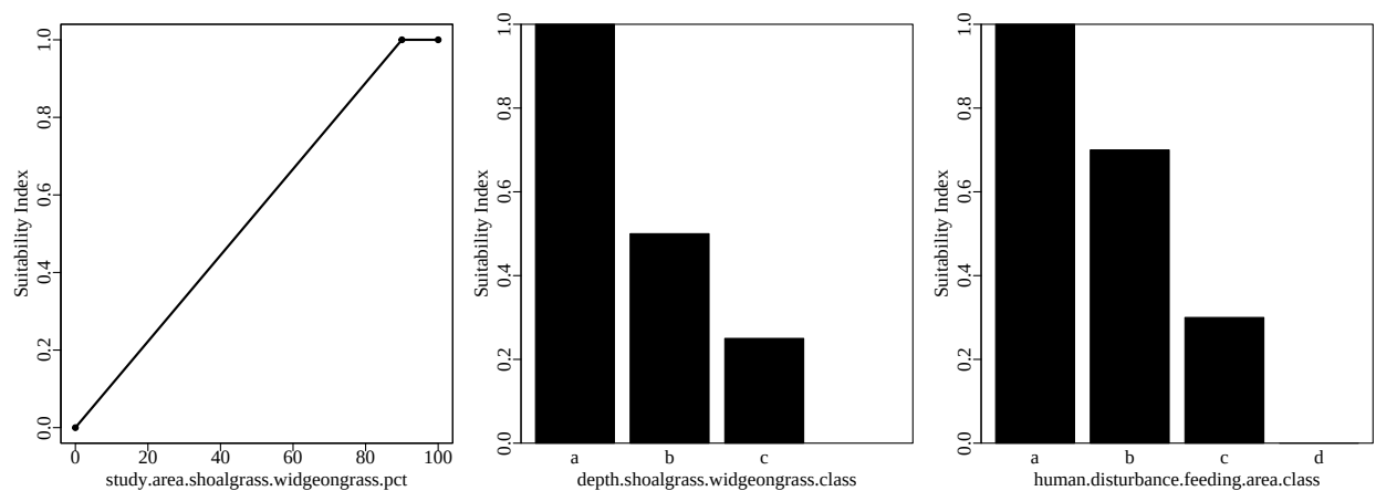
Figure 1. Suitability index graphs for variables included in the redheadWinteringWtrNotAvailable model in ecorest.
